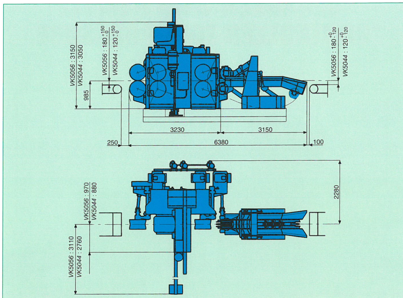
Main dimensions (mm)
